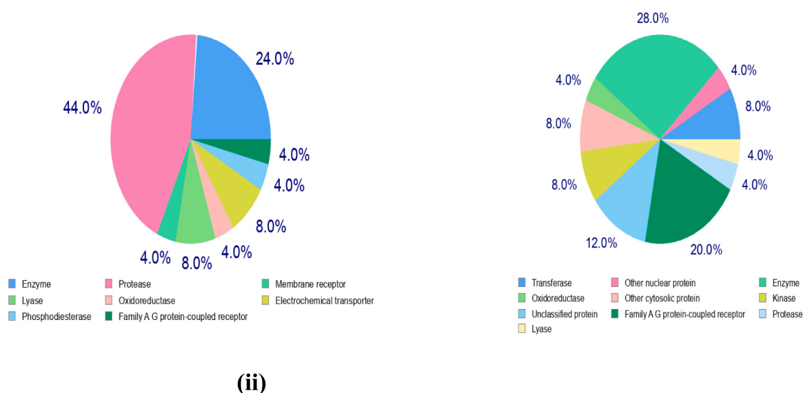
Fig. 12. Target Prediction of (i) NR and (ii) NMN.
