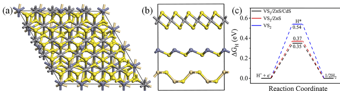
FIG. 7. (a) Top and (b) side view of VS 2 /ZnS/CdS heterostructure and (c) the free energy diagram of HER the pristine and heterostructures.
