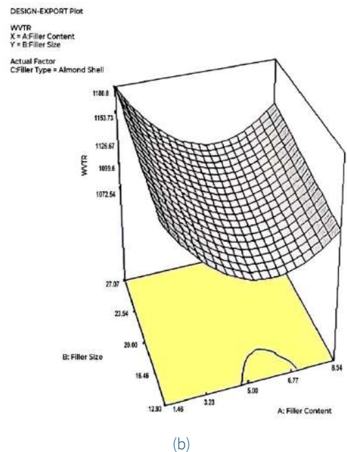
Figure 6. Effect of filler size and content on WVTR (a) walnut shell (b) almond shell.
