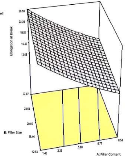
DESIGN-EXPORT Plot Elongation at Break X = A:Filler Content Y = B:Filler Size Actual Factor C:Filler Type = Almond Shell
