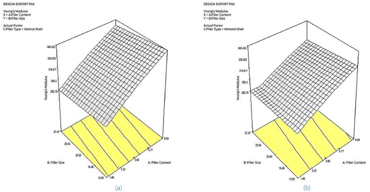
Figure 3. Effect of filler size and content on Young's modulus (a) walnut shell (b) almond shell.
