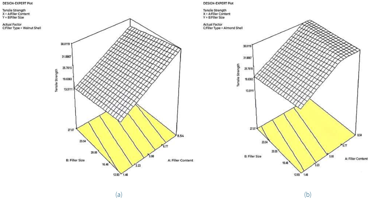
Figure 2. Effect of filler size and content on tensile strength (a) walnut shell (b) almond shell.
